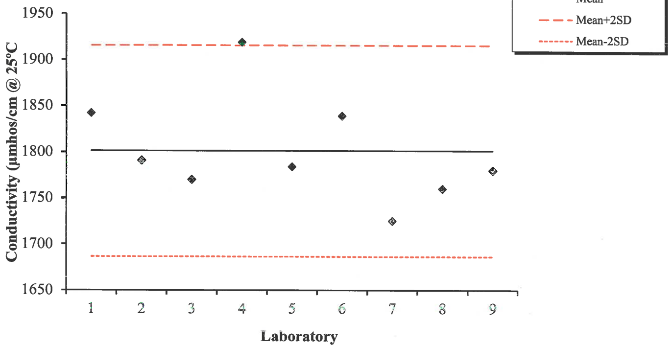
Figure 7: 2019 Performance Evaluation Conductivity Results Solution G
