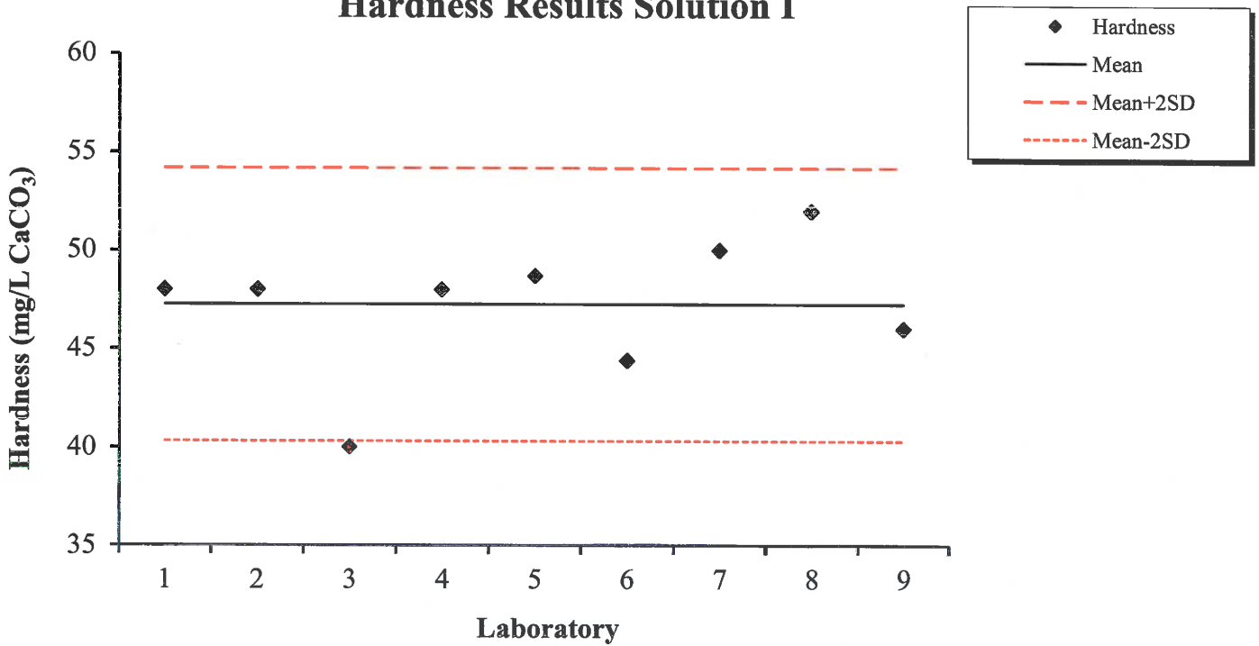
Figure 9: 2019 Performance Evaluation Hardness Results Solution I
