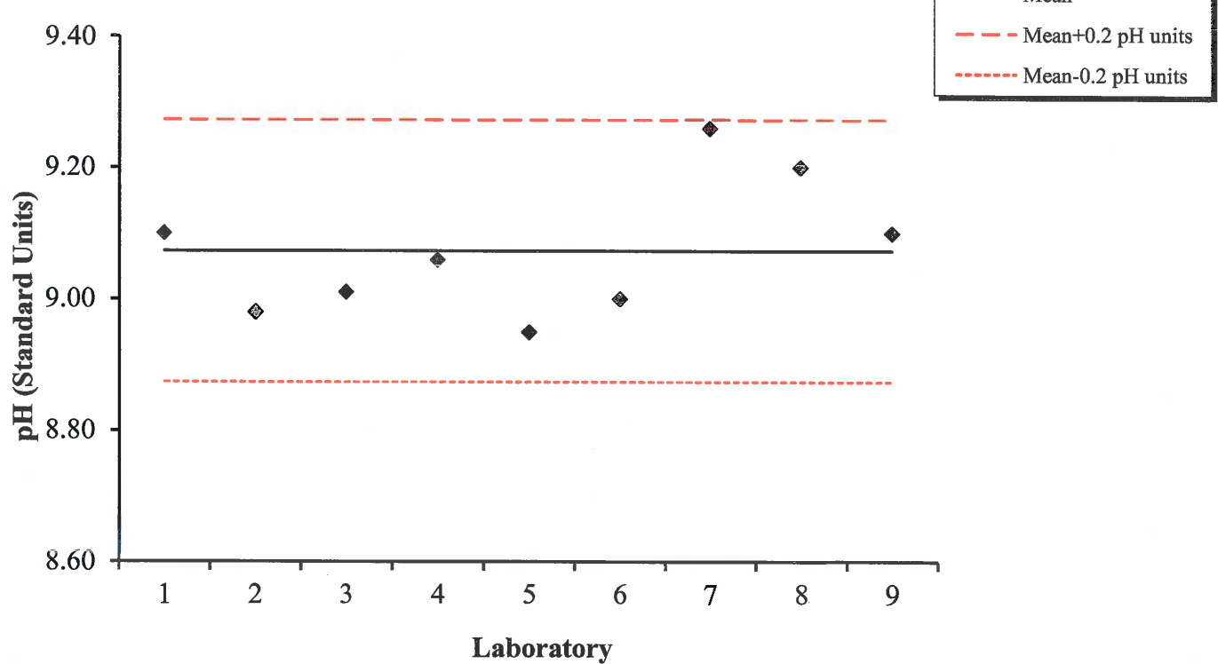
Figure 5: 2019 Performance Evaluation pH Results Solution E
