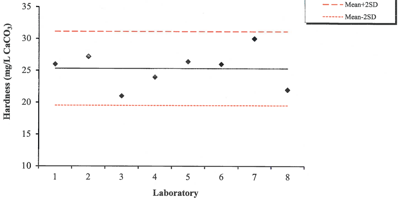
Figure 8: 2019 Performance Evaluation Hardness Results Solution H
