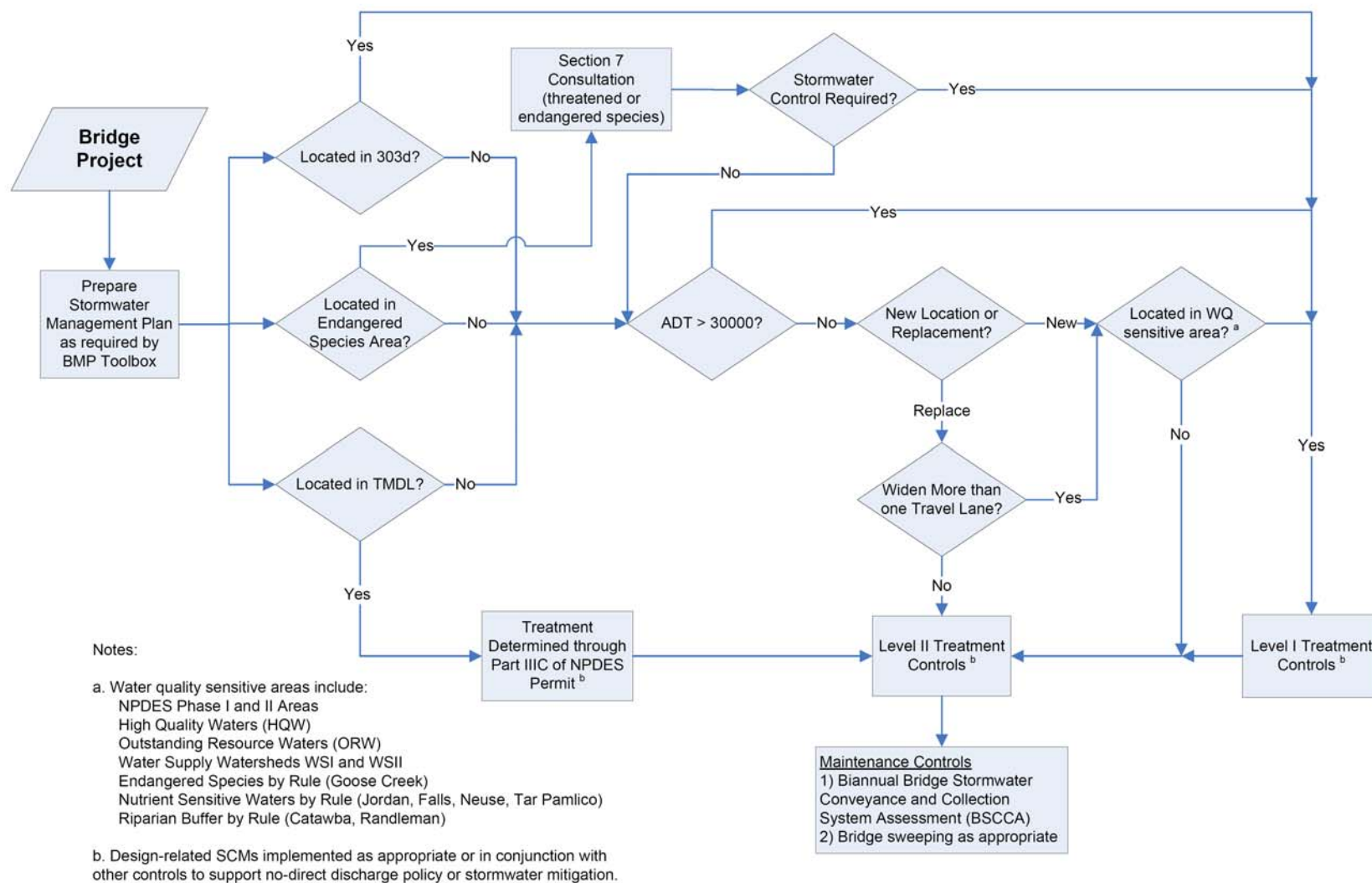
Figure 6.4-1: Process for estimating the number of SCMs implemented at new location and replacement bridges over waterways.
