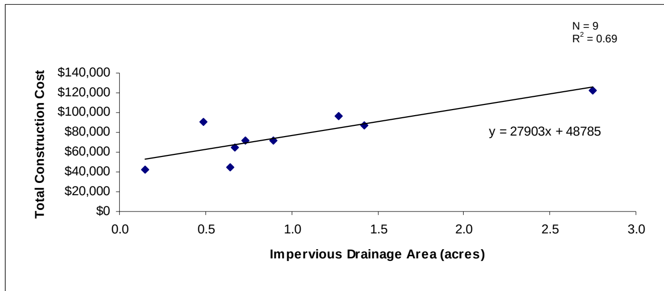
Figure 7.2-1: Comparison of bioretention basin construction cost to impervious drainage area.
